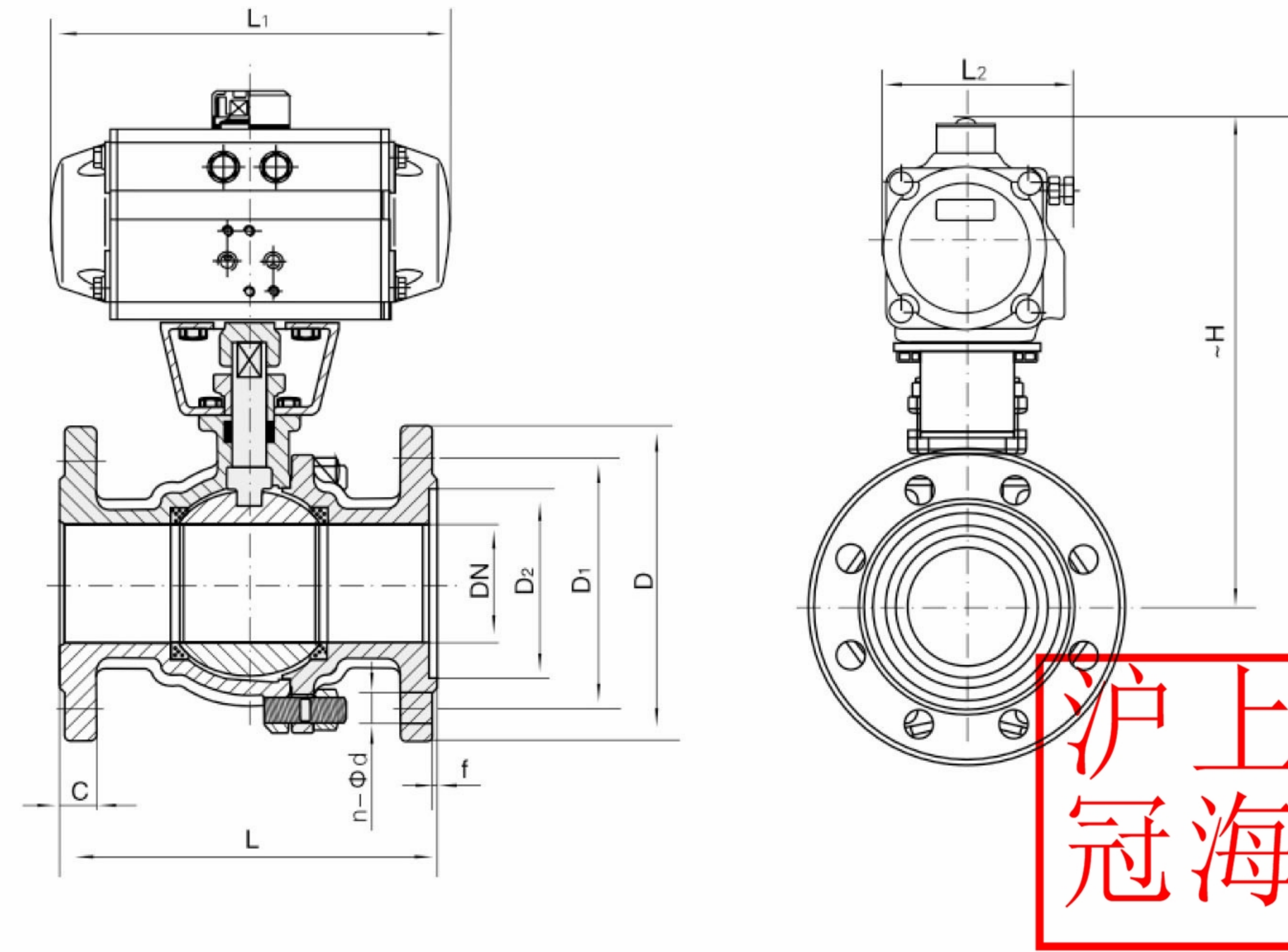
主要外形及连接法兰尺寸Q641F(N、P、H、Y)-Class 150 Main Outline and Connecting Flange Size
